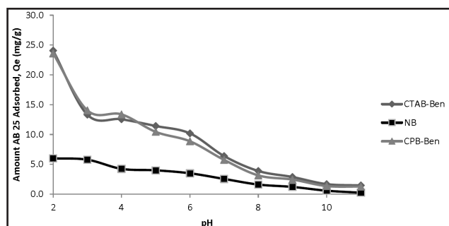
Figure 5: Effect of pH on the adsorption of AB 25 on NB, CTAB-Ben and CPB-Ben.
