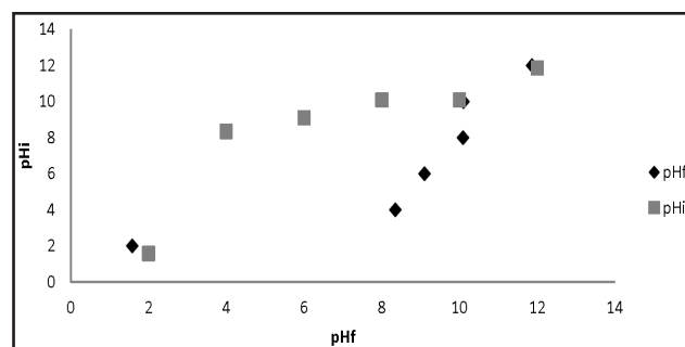
Figure 6: Dependence of pHf on pHi during equilibrium of 0.1g of CTAB-Ben and CPB-Ben with KCl to determine PZC.
