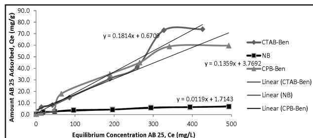
Figure 7: Equilibrium concentrations on the adsorption of AB 25 on CTAB-Ben, CPB-Ben and NB.
