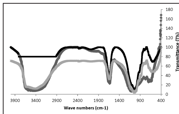
Figure 2: FTIR patterns of NB, CTAB-Ben and CPB-Ben.
