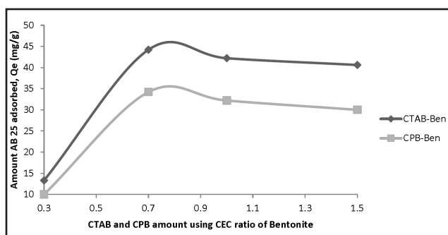
Figure 1: Relationship between amount of CTAB-Ben and CPB-Ben with amount of AB 25 adsorbed.
