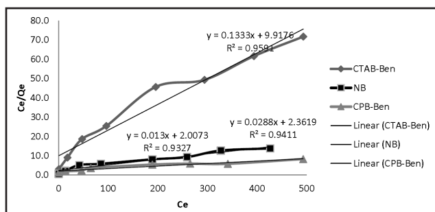
Figure 9: Langmuir isotherm graph for NB, CTAB-Ben and CPB-Ben.
