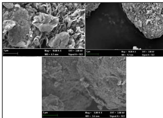
Figure 4: FESEM micrographs on CPB-Ben (left), CTAB-Ben (right) and NB (below).
