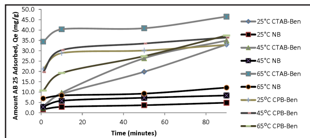
Figure 8: Test effects of temperature and time on the adsorption of AB 25 on CTAB-Ben, CPB-Ben and NB.
