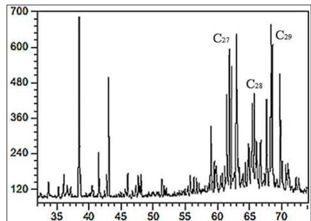
Figure 6: Biomarker analyses for crude oil from well Zubair-4 which represents Group 2A. Figure shows the analyses of m/z 217 steranes (Al-Ameri et al. , 2009).
