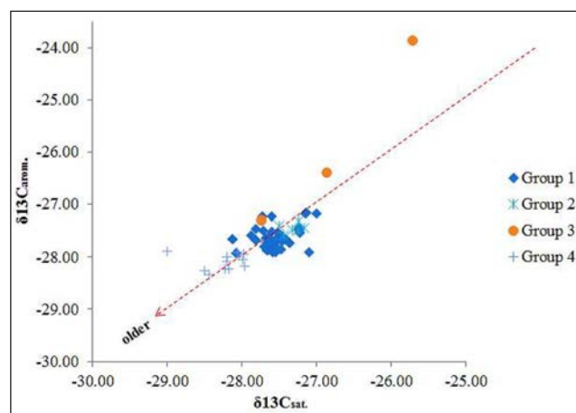
Figure 13: Plot of \delta^{13}C saturates versus \delta^{13}C aromatics for oils from Southern Mesopotamian Basin, Iraq. The plot separates oils and shows their relative ages.
