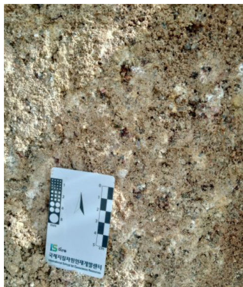
Figure 4: Exposed C1 horizon showing mottled, yellowish to brownish in colour with appearance of relict feldspar minerals and traces of biotite.
