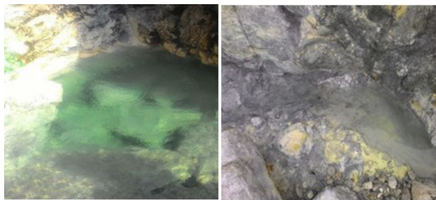
Figure 4: Geothermal manifestation of Siogung - Ogung area.
