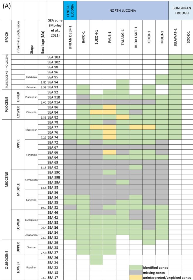
Figure 4: Well stratigraphic summaries across Sarawak Basin. (A) Well stratigraphic summary in Bunguran Trough, North Luconia and Central Luconia (Jintan Deep-1), based on the biostratigraphic zonation scheme of Morley et al. (2021). Note the main continuous interval of missing zones around the Middle Miocene (biozones ranging from SEA 46 to SEA 72 equivalent to ~17.5 to 8.2 Ma). Based on data compiled from internal PETRONAS reports. (B) Nannofossil biozones (Martini, 1971) in selected wells, showing missing NN zones at the MMU, especially NN6 to NN8, amounting to ca. 2–3 Myr hiatus in Central and SW Luconia. At Talang and Bukoh-1 in North Luconia, the hiatus is even larger, from NN4 to NN8, or around 6.5 Myr. (C) Planktonic foraminifera biozones (Blow, 1969) identified in selected wells, showing missing N zones (N10-N13) equivalent duration of 1.5 to 5.5 Myr at the MMU. All charts were compiled from internal reports (Iyer, 2015). Well locations are shown in Figure 3.
