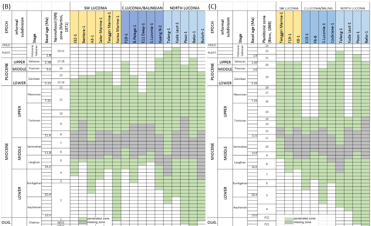
Figure 4: Well stratigraphic summaries across Sarawak Basin. (A) Well stratigraphic summary in Bunguran Trough, North Luconia and Central Luconia (Jintan Deep-1), based on the biostratigraphic zonation scheme of Morley et al. (2021). Note the main continuous interval of missing zones around the Middle Miocene (biozones ranging from SEA 46 to SEA 72 equivalent to ~17.5 to 8.2 Ma). Based on data compiled from internal PETRONAS reports. (B) Nannofossil biozones (Martini, 1971) in selected wells, showing missing NN zones at the MMU, especially NN6 to NN8, amounting to ca. 2–3 Myr hiatus in Central and SW Luconia. At Talang and Bukoh-1 in North Luconia, the hiatus is even larger, from NN4 to NN8, or around 6.5 Myr. (C) Planktonic foraminifera biozones (Blow, 1969) identified in selected wells, showing missing N zones (N10-N13) equivalent duration of 1.5 to 5.5 Myr at the MMU. All charts were compiled from internal reports (Iyer, 2015). Well locations are shown in Figure 3.
