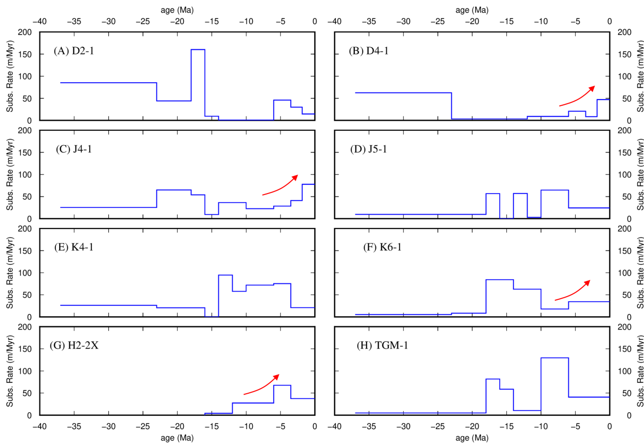
Figure 10: (A) – (H) Basement subsidence rate curves based on tectonic subsidence at well locations to the south of Bunguran Trough, mainly in SW Luconia and Balingian provinces. Well data from Madon et al. (2013) were re-calculated based on updated stratigraphy (Morley et al. , 2021).
