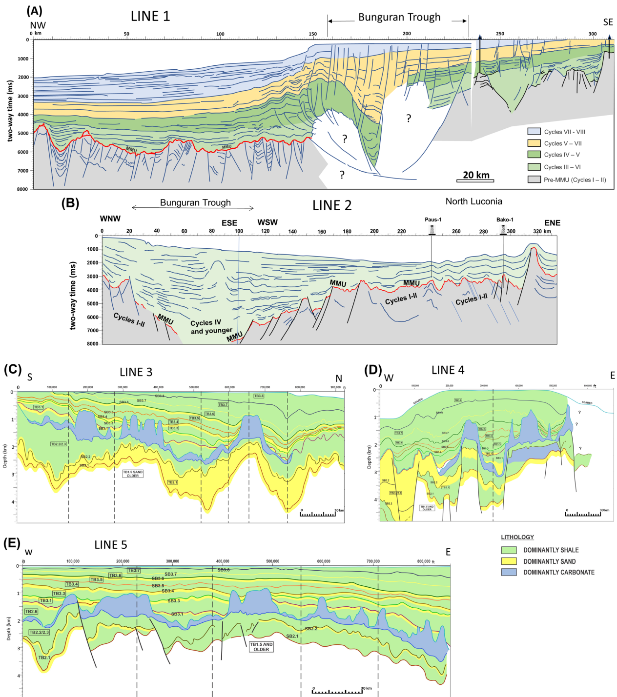
Figure 6: Geoseismic profiles across Sarawak Basin, depicting the main structural and stratigraphic features. Profile locations are shown by red lines on the map in Figures 1 and 5. (A) Line 1: NW-SE profile crossing the western Sarawak Shelf and Bunguran Trough, showing the post-MMU prograding shelf-slope sediments over highly deformed Cycles I-II sequences. (B) Line 2: WNW-ESE profile crossing Bunguran Trough and North Luconia, showing the deep Bunguran Trough and onlapping post-MMU (Cycle IV and younger) sediments filling the trough as well as draping the rifted Middle Miocene paleo-topography. (C) Line 3: Crossing the Central Luconia in roughly N-S direction, showing the prograding shelf sediments downlapping onto the basal carbonate surface upon which carbonate build-ups developed. (D) Line 4: W-E line crossing the northern part of Central Luconia separating the deep basin on either side (West Luconia and Baram deltas). (E) Line 5, also oriented W-E across the central part of Central Luconia showing the extended pre-Cycle IV section overlain by Cycle IV-V carbonate build-ups. The effect of sediment loading in Baram Delta to the east is indicated by the monoclinical pre-carbonate strata and expanded stratigraphic thicknesses in the post-carbonate section. Lines 1 and 2 were modified from Madon & Jong (2022); Lines 3, 4 and 5 from Taylor et al. (1977).
