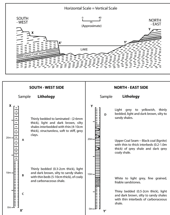
Figure 2: Geological cross-sections and locations of samples. (Points X and Y are shown in Figure 1).
