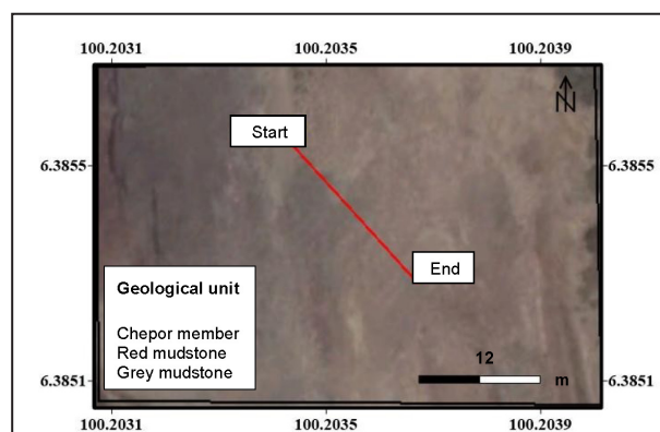
Figure 3: Location of the survey line from top view (Google earth, 2016).
