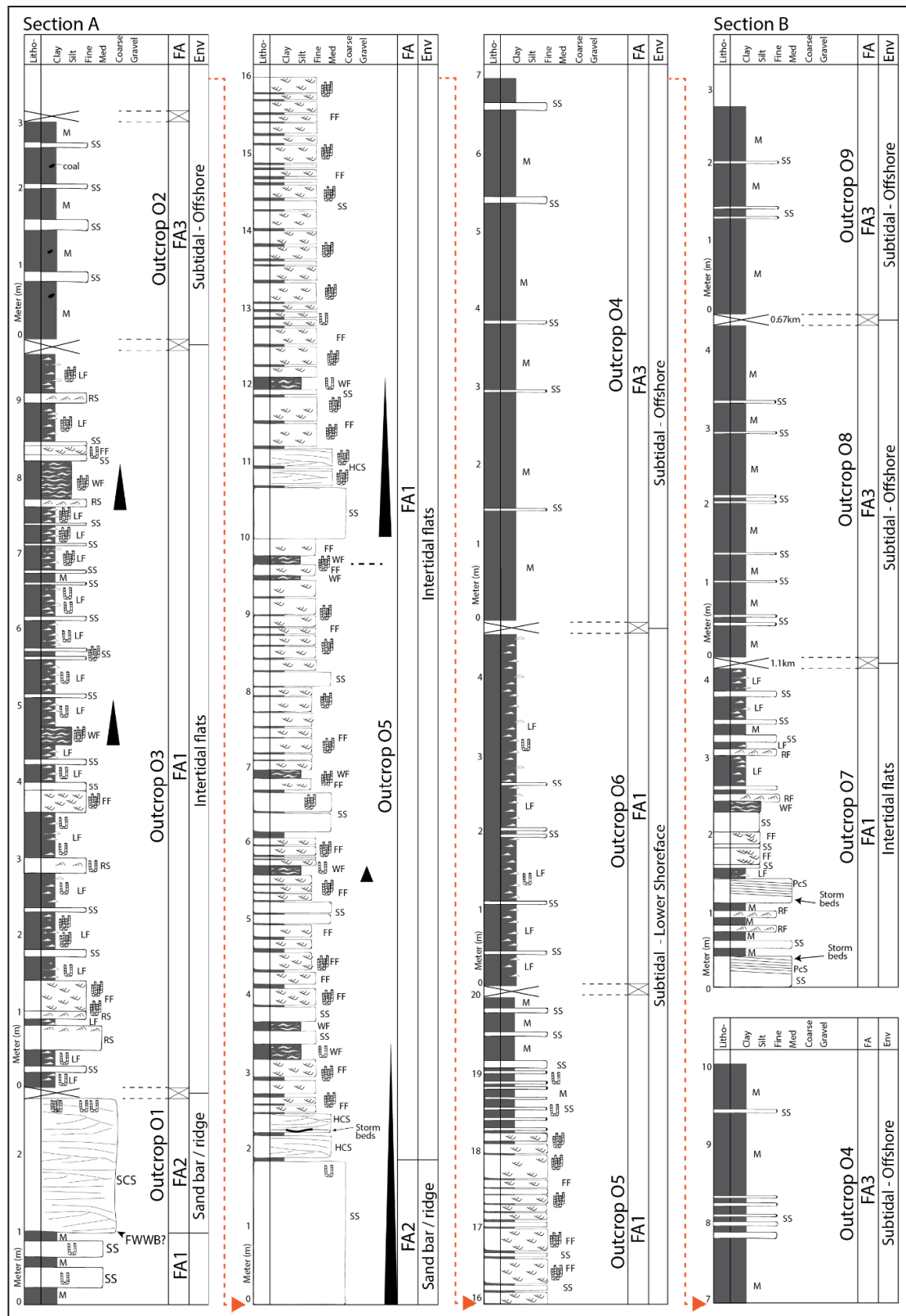
Figure 3: Correlated sedimentary logs of Tanjong Formation at Imbak Canyon, Tongod, Sabah.
