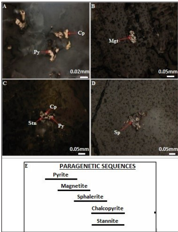
Figure 3: Photomicrograph of a polished section of the granite rock sample TBL-21MN/02B/R, Tobaoli, consisting of pyrite (Py) 2%, and chalcopyrite (Cp) < 0.5% (A), magnetite (Mgt) (trace) (B), stannite (Stn) (< 0.5%), chalcopyrite < 0.5%, and pyrite (C), sphalerite (Sp) (trace) (D). It appears that chalcopyrite and stannite are intergrowths.
