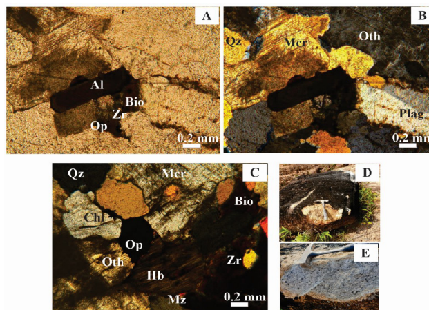
Figure 2: Photomicrograph of thin section sample TBL-21MN/2B/R, Klabat Granite. A. Plane polarized light, showing biotite (Bio) with elongated blackish-brown of sub-euhedral crystal, allanite (Al) with euhedral elongated crystal, opaque minerals (Op), and fine grain of zircon (Zr) with bright yellow. B. Cross Nicol, showing microcline (Mcr) with irregular brownish-yellow crystal, plagioclase (Plag) with prismatic twin crystal, orthoclase (Oth) with pale gray, and quartz (Qz) with yellow anhedral crystal. C. Cross Nicol, showing quartz (Qz), microcline (Mcr), orthoclase (Oth), biotite (Bio), hornblende (Hb) with dark greenish-brown, chlorite (Chl) with blackish-white, zircon (Zr) with yellow sub-euhedral crystal, monazite (Mz) with bright pinkish-yellow, and opaque minerals has euhedral crystal. D. Boulder of mineralized granite from the basement of laterite profile. E. Sample of granite boulder consists of quartz, feldspar, biotite, and a little hornblende.
