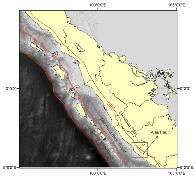
Figure 1: The location of the Alas Fault and the Bengkulu Segment of the Sumatran Fault shown in the black box. Administratively, the research area is in Seluma Regency, Bengkulu, Indonesia. Geographically, the research area is located at coordinates 48 260385 E 9540068 S and 48 269490 E 9521092 S with an area of \pm 1,503.03 \text{ km}^2 (Modified from Daryono et al. , 2019).
