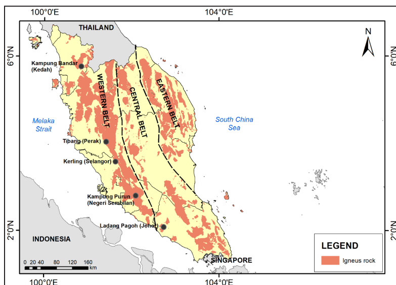
Figure 1: Map showing the granite belts in Peninsular Malaysia.
