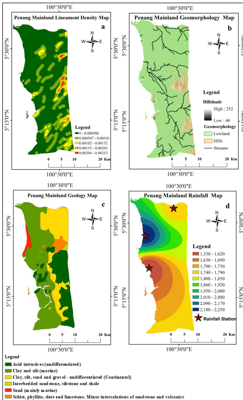
Figure 5: Thematic layers of (a) Lineament Density Map ( \text{m}/\text{m}^2 ), (b) Geomorphology Map, (c) Geology Map, (d) Rainfall Map (mm) of Penang mainland.
