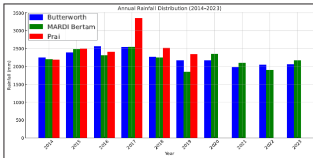
Figure 3: Annual rainfall distribution (mm) at Butterworth, Mardi Bertam, and Prai stations, 2014–2023.
