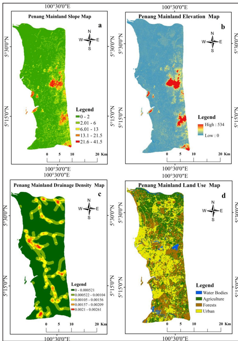
Figure 6: Thematic layers of (a) Slope Map ( ^{\circ} ), (b) Elevation Map (m), (c) Drainage Density Map ( \text{m}/\text{m}^2 ), and (d) Land Use/Land Cover Map) of Penang mainland.
