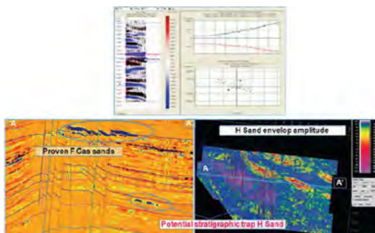
Figure 3: Fluid properties prediction by using AVO analysis has found potential stratigraphic trap in H sand of B field.
