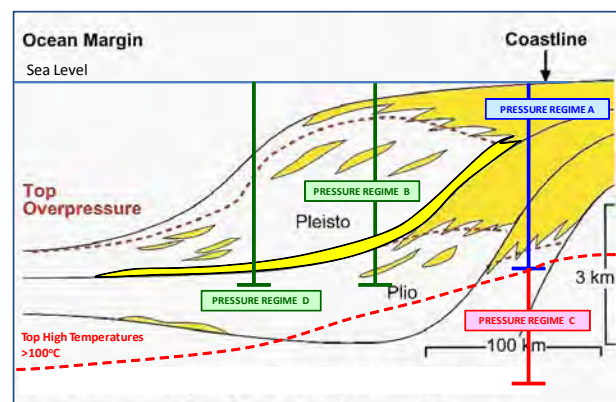
Figure 1: Location of Pressure Regimes A-D in a typical deltaic environment.
