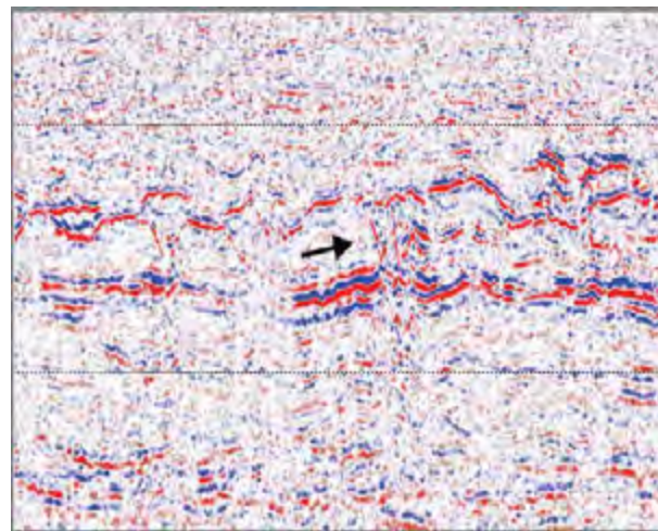
Figure 2: Cross section of seismic migrated stack trace data volume showing steeply dipping events, interpreted as sandstone injectites (arrow), (Source: McHugo et al., 2003)
