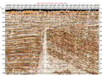
Figure 2: Removal of artifacts using AZNMO.
