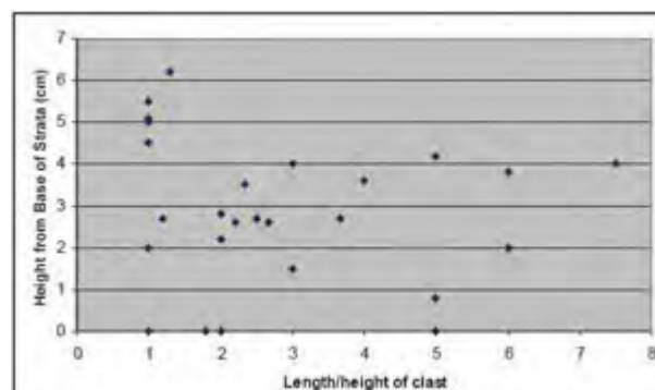
Figure 3: Variations of mean dimensions of clasts as a function of vertical distance from the base of the strata.
