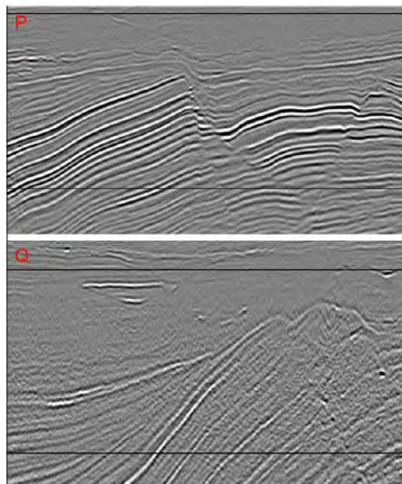
Figure 2: Migrated stacked sections showing structures from South China Sea. Top – 2D SRME has been effective. Bottom – residual multiple of shallow diffractions remains. NB. Data are from the same survey, with the same processing sequence applied and the structures are approximately 30km apart.
