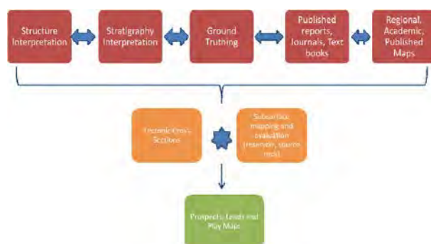
Figure 4: Satellite based evaluation workflow that leads to prospective corner identification.
