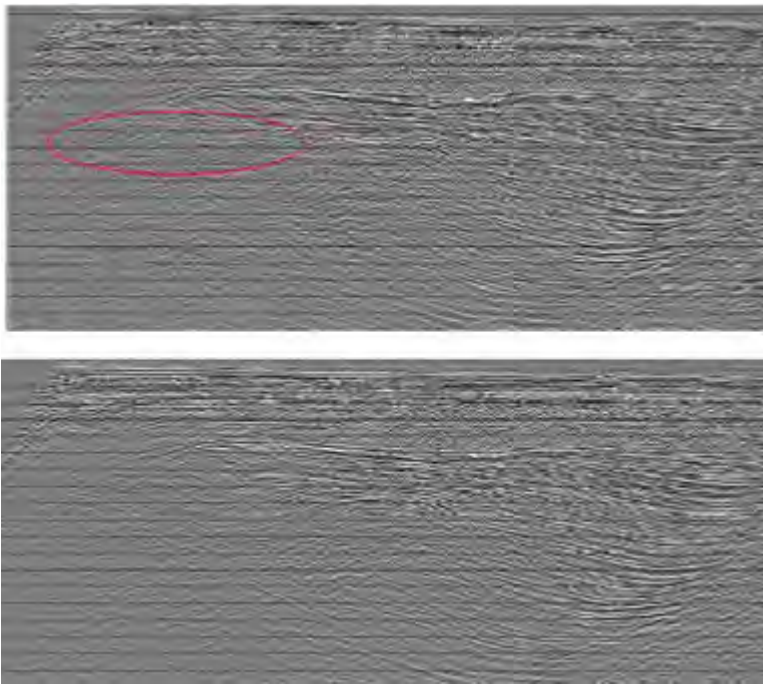
Figure 4: Difference between input stacked section (Figure 3) and stack with 2D SRME applied after trace drop to the annotated trace spacing. A significant deterioration in effectiveness of the multiple attenuation is noted between 18.75m and 25.0m which matches our prediction.
