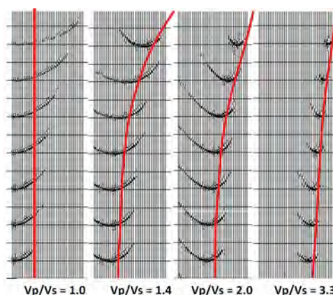
Figure 4: P-S impulse response.
