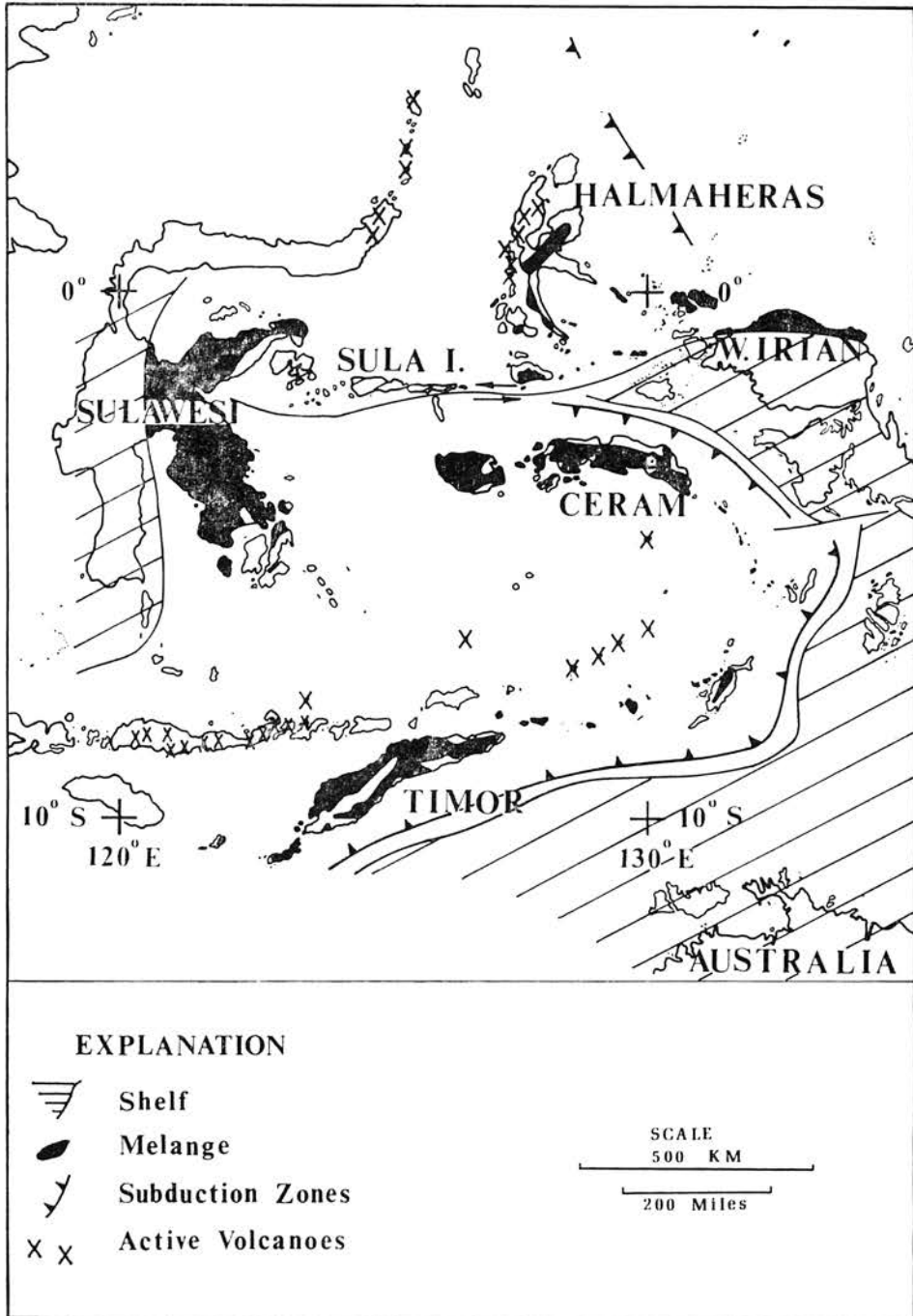
Fig. 1. Generalised Tectonic Map of the Moluccas.
