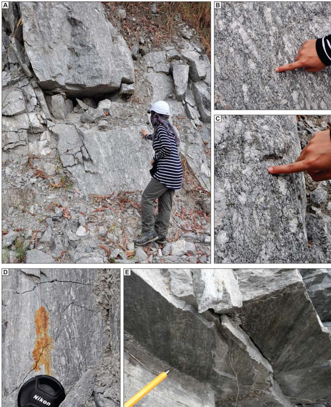
Figure 5: Main Range Granite Province rocks exposed near Kampung Jaya Sepakat [397277 327485], southwest of Kuala Lumpur (Locn2, Figure 2); showing the range of well-developed pre- and post-full crystallisation fabrics, including mylonitic granite: A, B) elongate quartz and K-feldspar megacrysts in foliated granitic rocks; C) elongate grey, semipelitic xenolith aligned within pre-full crystallisation fabric; D) intensely foliated granitic mylonite, fabric encloses strongly sigmoidal porphyroclasts of quartz and K-feldspar; E) intensely lineated granitic mylonite, down-to-north transport, down-dip and away from the viewer. The foliation dips 68° to 020°N; the lineation in E plunges 60° towards 342°N. View is generally to north for all frames. All images BGS © UKRI 2020.
