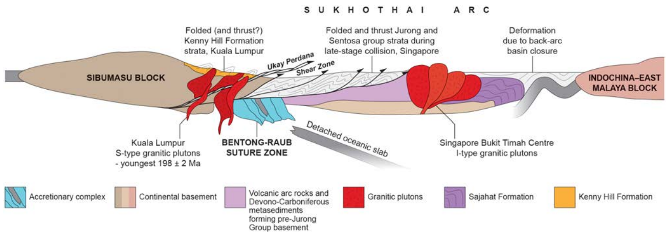
Figure 8: Cartoon showing the tectonic evolution of the Singapore/Kuala Lumpur crustal region during late Triassic to earliest Jurassic times when subduction was generally north-directed; the section therefore has a general N-S alignment at that time. This representation relates to the orogenic deformation in this now southern sector of Sibumasu and the Sukhothai Arc, and the amalgamation of Sundaland (after Sone & Metcalfe, 2008). The Sibumasu and Indochina-East Malaya blocks are shown in simplified form (see also Metcalfe, 2017 for details of these elements). The Ukay Perdana Shear Zone (UPSZ) identified in north-eastern Kuala Lumpur is proposed as a marker for a major crustal boundary between the leading edge of the Sibumasu Block (Kuala Lumpur) and the now-shortened forearc basin of the Sukhothai Arc (Singapore). The accretionary Bentong-Raub Suture Zone was probably over-riden in these later stages of collision and amalgamation. BGS © UKRI 2020
