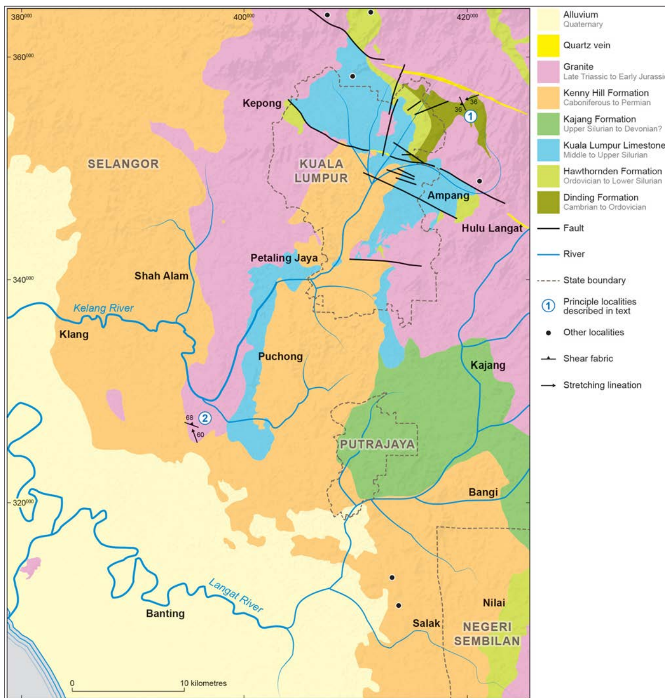
Figure 1: General geological map of Kuala Lumpur, the principal locations described in the text are superimposed (after Jabatan Mineral dan Geosains Malaysia, 2011). The principle localities at Jalan Ukay Perdana 4 [420155 354436] and Kampung Jaya Sepakat [397277 327485] are numbered (1 and 2 respectively); other localities discussed in the text and illustrated in Figure 4 are located as black dots.
