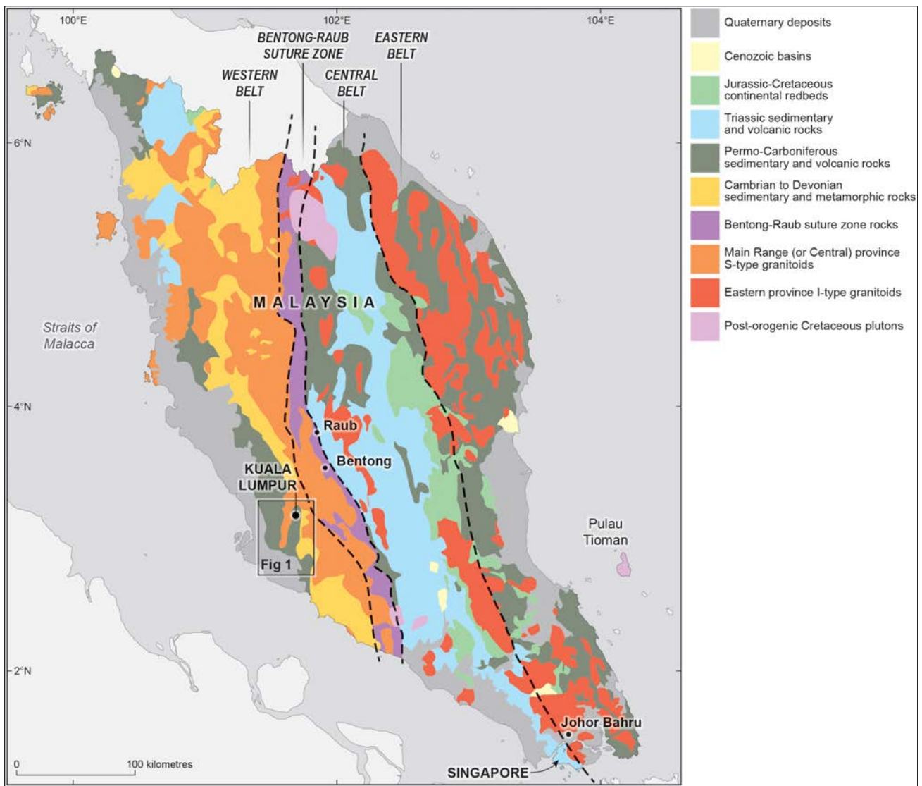
Figure 2: Simplified regional geological map of Peninsular Malaysia. The map shows the limits of the tectono-stratigraphical Western, Central and Eastern belts, and the trace of the BRSZ that marks the orogenic suture between Sibumasu (Western Belt) and the Sukhothai Arc (Central and Eastern belts); (after Metcalfe, 2013). The BRSZ apparently passes some c. 50 km east of Kuala Lumpur and c. 100 km west of Singapore; boxed area, including Kuala Lumpur, is shown in more detail in Figure 1.
