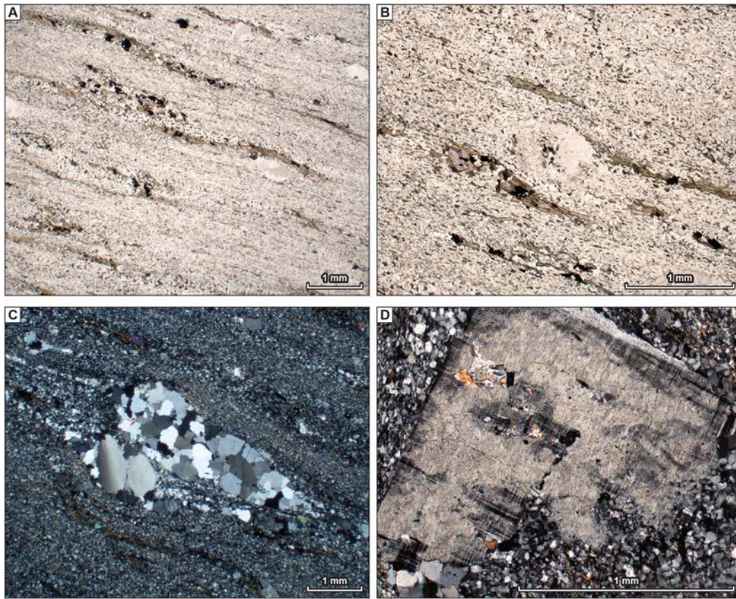
Figure 7: Intensely foliated granitic ultramylonite, Jalan Ukay Perdana 4 [420155 354436], thin section views. A) Thoroughly annealed granoblastic aggregates of quartz, orthoclase and oligoclase; prisms of fresh muscovite and biotite grow along the quartzo-feldspathic grain boundaries and are very strongly aligned within the mylonitic fabric. B) Biotite-rich layers define bands within the foliation spaced at c. 1 mm; in these micaceous layers micas are up to 0.25 mm long. C) Stretched and polygonised quartz porphyroclasts may be up to 4 mm long within the foliation, and c. 1 mm wide, sigmoidal in overall form and swept around by the mica fabric; these quartz porphyroclasts are always composed of sub-grains with conspicuously lobate-cusped migrating sub-grain. D) K-feldspar porphyroclasts are blocky in form though still swept by (and abraded within) the enclosing mylonitic fabric and locally retain evidence of coarsely perthitic exsolution textures comprising intergrowths of orthoclase and microcline. All images BGS © UKRI 2020.
